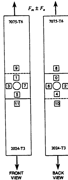
Figure 2. Spot-welded lap-joint specimen instrumented with 12 PZT wafer transducers. The numbers represent the transducer stations arranged in flip-side pairs on the specimen. During the fatigue tests, the applied force has a mean component, F_m , and an alternating component, F_a .
