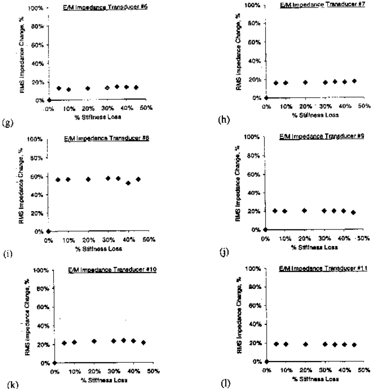
Figure 9 (continued). Correlation between RMS impedance change and specimen stiffness loss, as recorded by each transducer.
