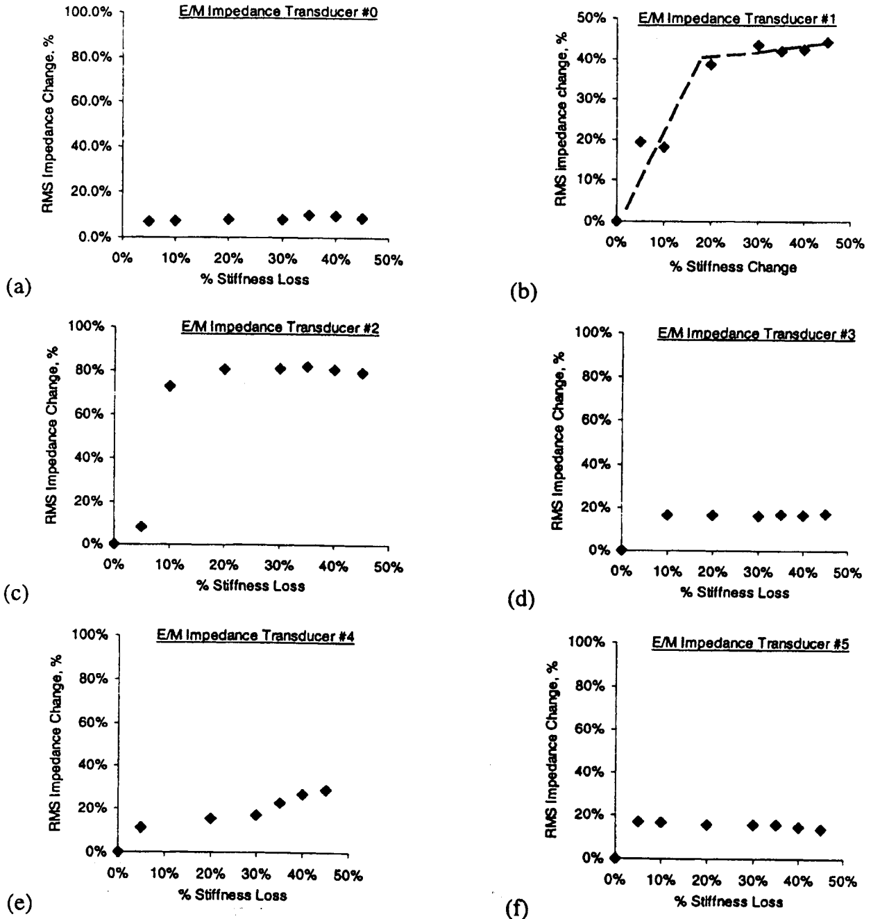
Figure 9. Correlation between RMS impedance change and specimen stiffness loss, as recorded by each transducer.
