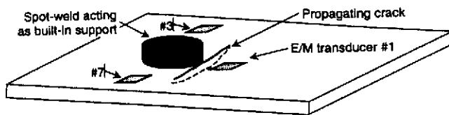
Figure 11. Representation of the bottom plate of the spot-welded lap-shear specimen with crack propagation close to the spot weld. The crack propagation radically changes the boundary conditions in its vicinity.
