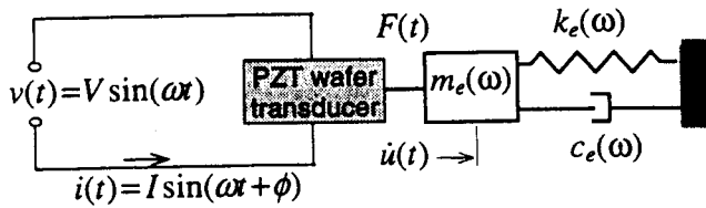
Figure 1. Electro-mechanical coupling between the PZT transducer and the structure.
