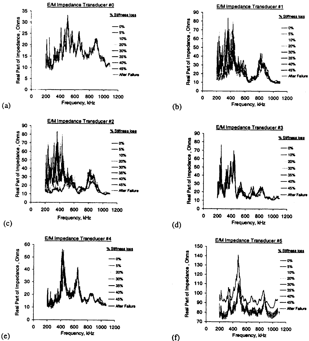
Figure 8. Superposed plots of impedance signatures of E/M transducers for increasing amounts of specimen stiffness loss (available for viewing in color at: http://www.engr.sc.edu/research/llmss/default.html ).
