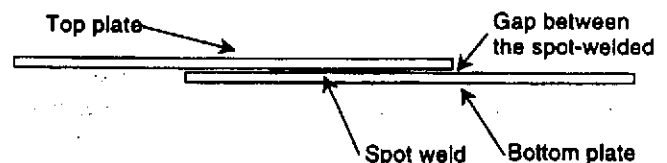
Figure 10. Side view of a spot-welded lap-shear specimen featuring the top and bottom plates, the spot weld, and the gap between the plates.
