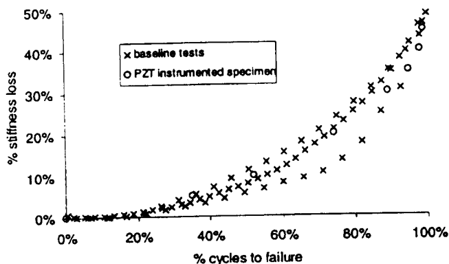
Figure 6. Graph of percentage stiffness loss vs. percentage cycles to failure for lap-shear spot weld specimens tested at P_{max} = 2.7 kN and R = 0.1 .
