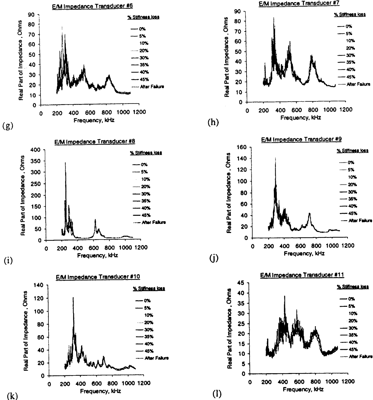
Figure 8 (continued). Superposed plots of impedance signatures of E/M transducers for increasing amounts of specimen stiffness loss (available for viewing in color at: http://www.engr.sc.edu/research/lamss/default.html ).
